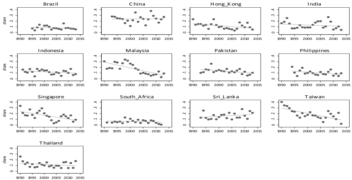
Figure 5: Covariance Share in non-OECD Countries
