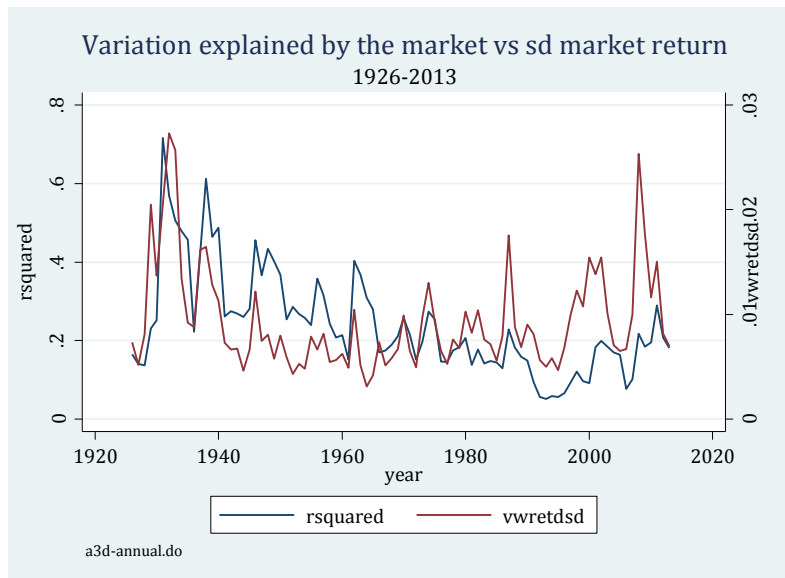
Figure 7: Variability of explanatory variable and R^2
