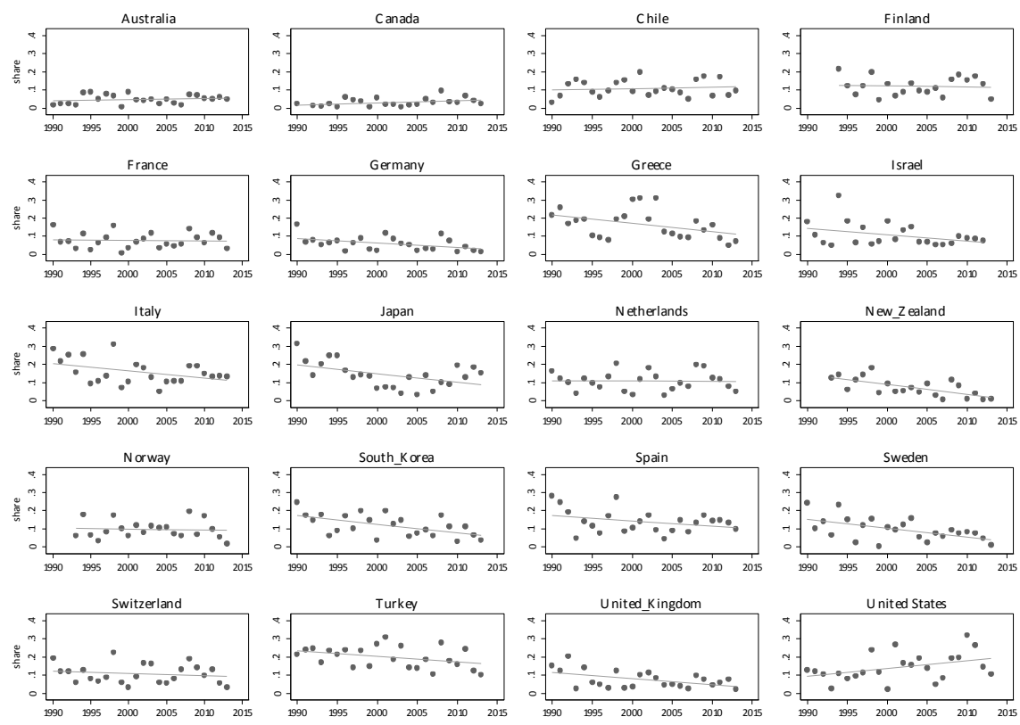
Figure 4: Covariance Share in OECD Countries
